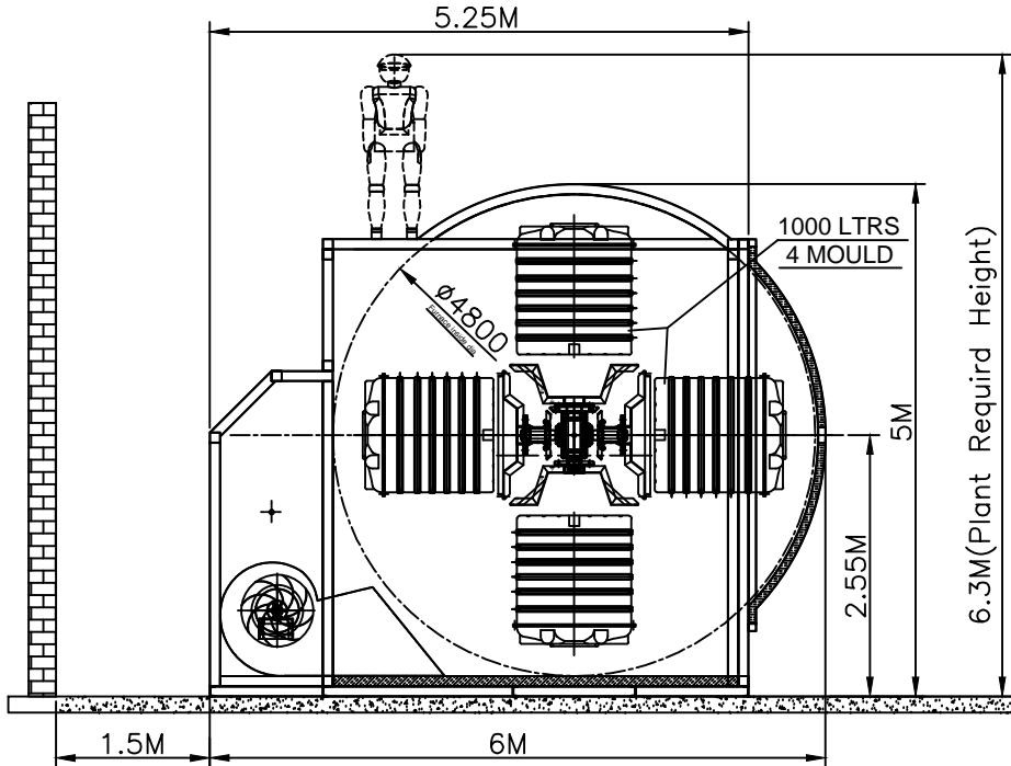
SIDE VIEW.
